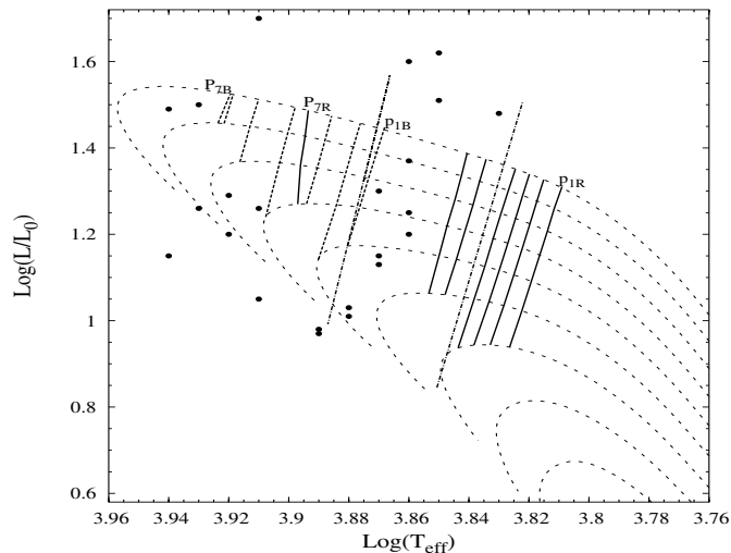
Figure 2: Blue and red edges of the PMS theoretical IS for radial modes from p_1 to p_7 for models with \alpha = 1.8 . Small points correspond to observations. Broken dotted lines give the IS of Marconi & Palla 1998.
