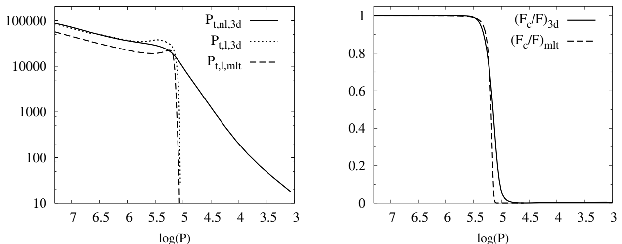
Figure 1: Turbulent pressure (left) and convective flux relative to total flux (right) as obtained with 3D hydrodynamic models (Stein & Nordlund 1998) and MLT.
